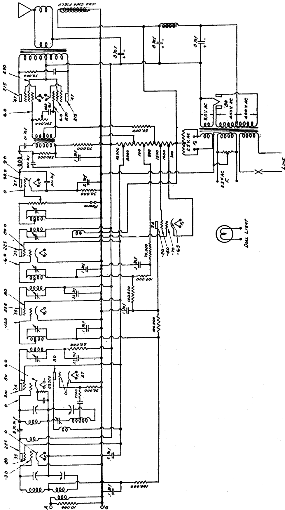
SCHEMATIC DIAGRAM OF LYRIC MODEL S-10 CHASSIS
